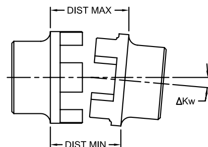
Angular Displacement
