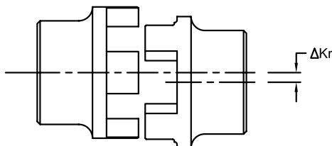
Radial Displacement
